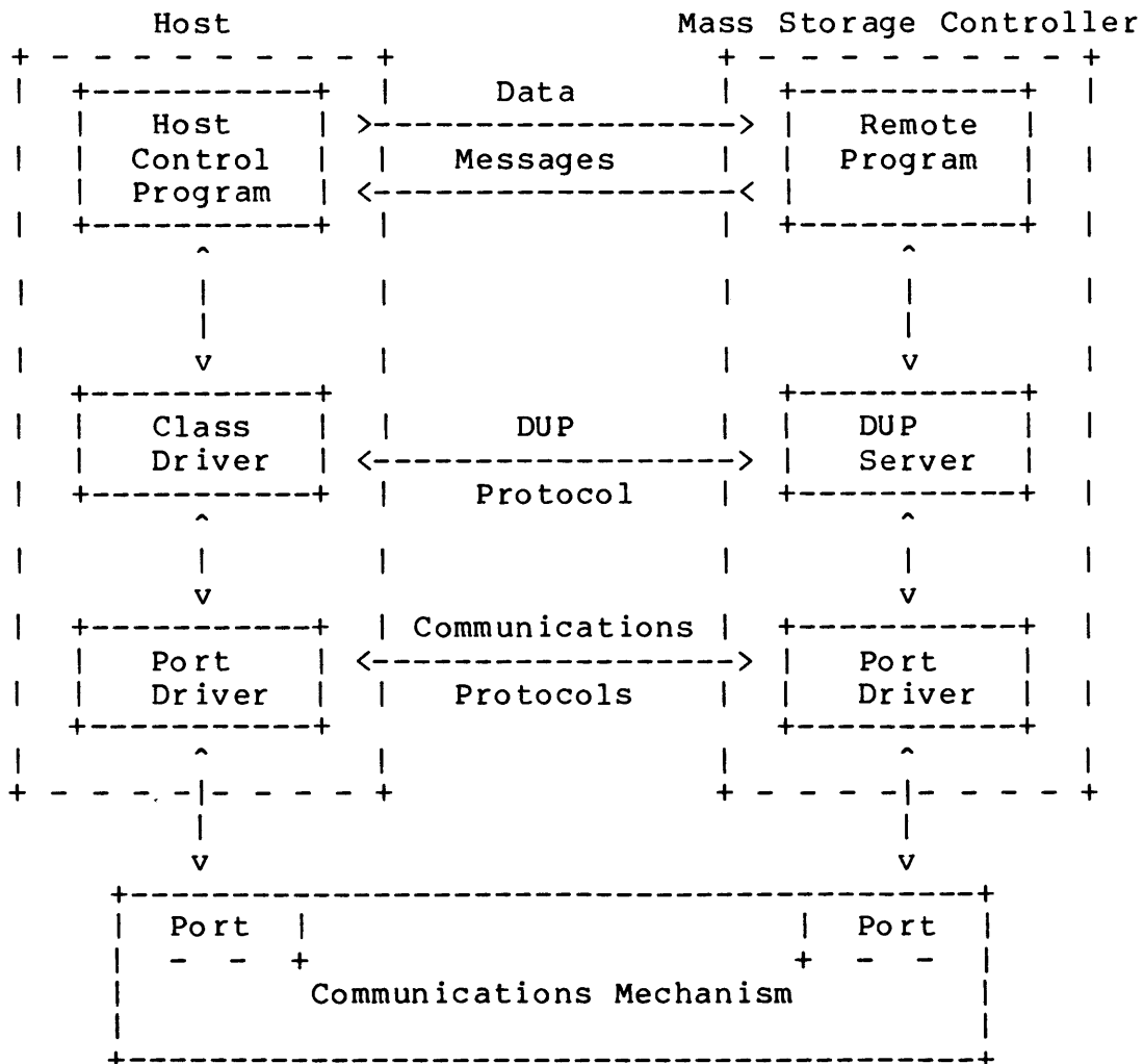
Figure 1-1 Example System
